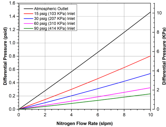
Mott GSMM-55-010-14 Flow Rate vs. Differential Pressure Typical Flow Curves as a Function of System Pressures
