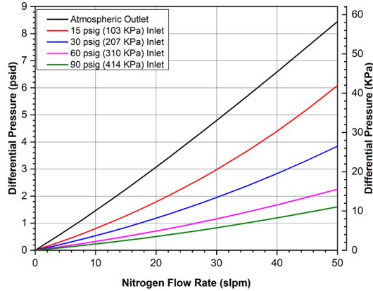
Mott GSMM-55-050-14 Flow Rate vs. Differential Pressure Typical Flow Curves as a Function of System Pressures
