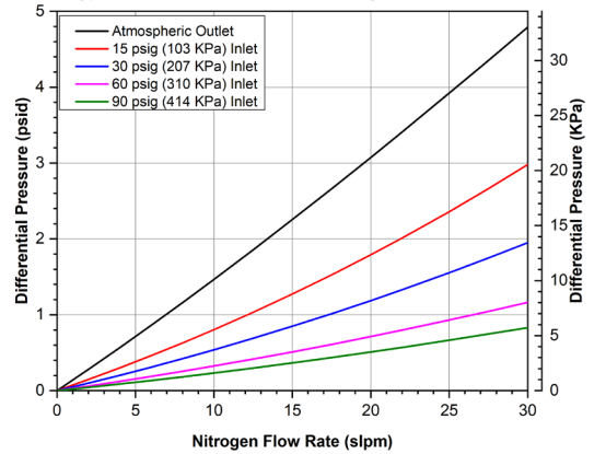
Mott GSMM-55-030-14 Flow Rate vs. Differential Pressure Typical Flow Curves as a Function of System Pressures
