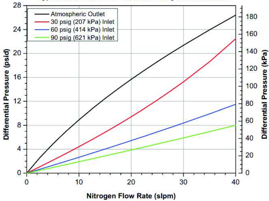
Mott POU-05-N Flow Rate vs. Differential Pressure Typical Flow Curves as a Function of System Pressures
