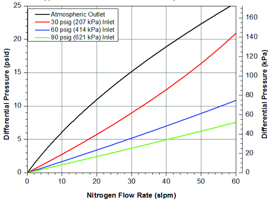
Mott POU-015-S Flow Rate vs. Differential Pressure Typical Flow Curves as a Function of System Pressures
