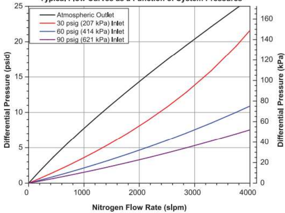
Mott DEF4000 Flow Rate vs. Differential Pressure Typical Flow Curves as a Function of System Pressures
