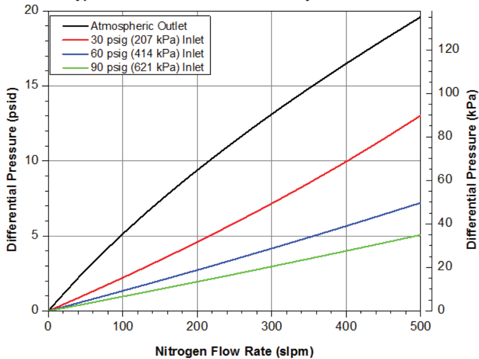
Mott GSP515H3 Flow Rate vs. Differential Pressure Typical Flow Curves as a Function of System Pressures
