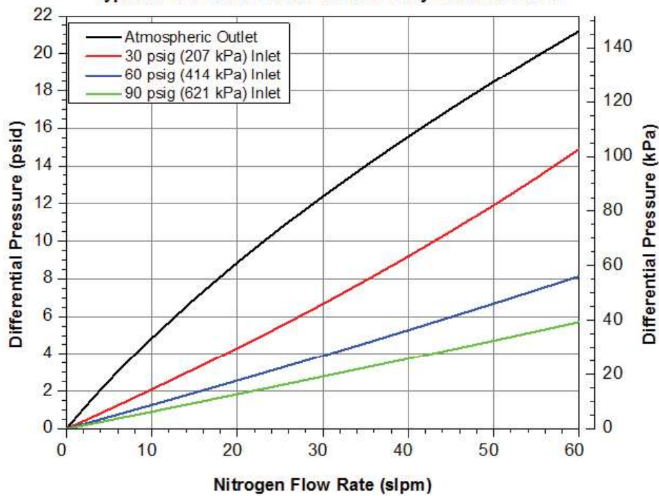
Mott GSP3752 Flow Rate vs. Differential Pressure Typical Flow Curves as a Function of System Pressures
