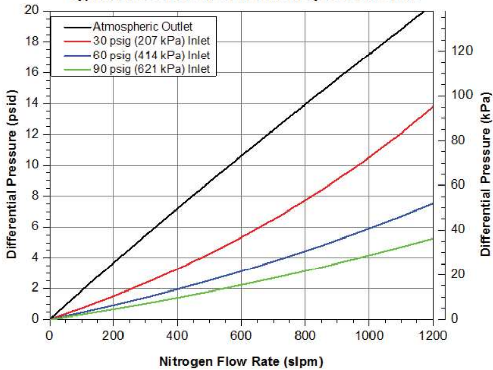
Mott GSP11215H3 Flow Rate vs. Differential Pressure Typical Flow Curves as a Function of System Pressures
