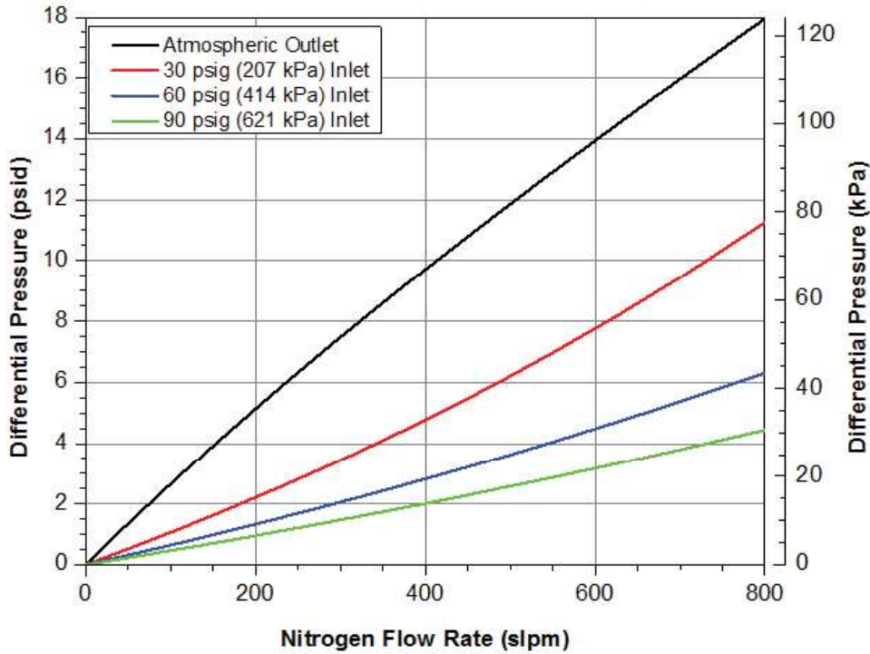
Mott GSP11215H1 Flow Rate vs. Differential Pressure Typical Flow Curves as a Function of System Pressures
