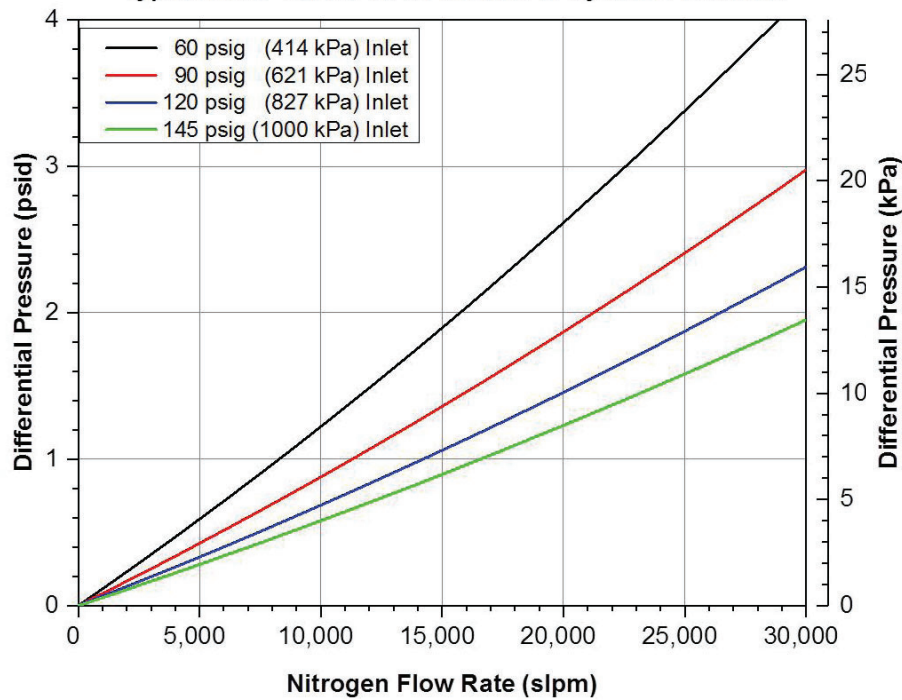
Mott BGF-610H Flow Rate vs. Differential Pressure Typical Flow Curves as a Function of System Pressures
