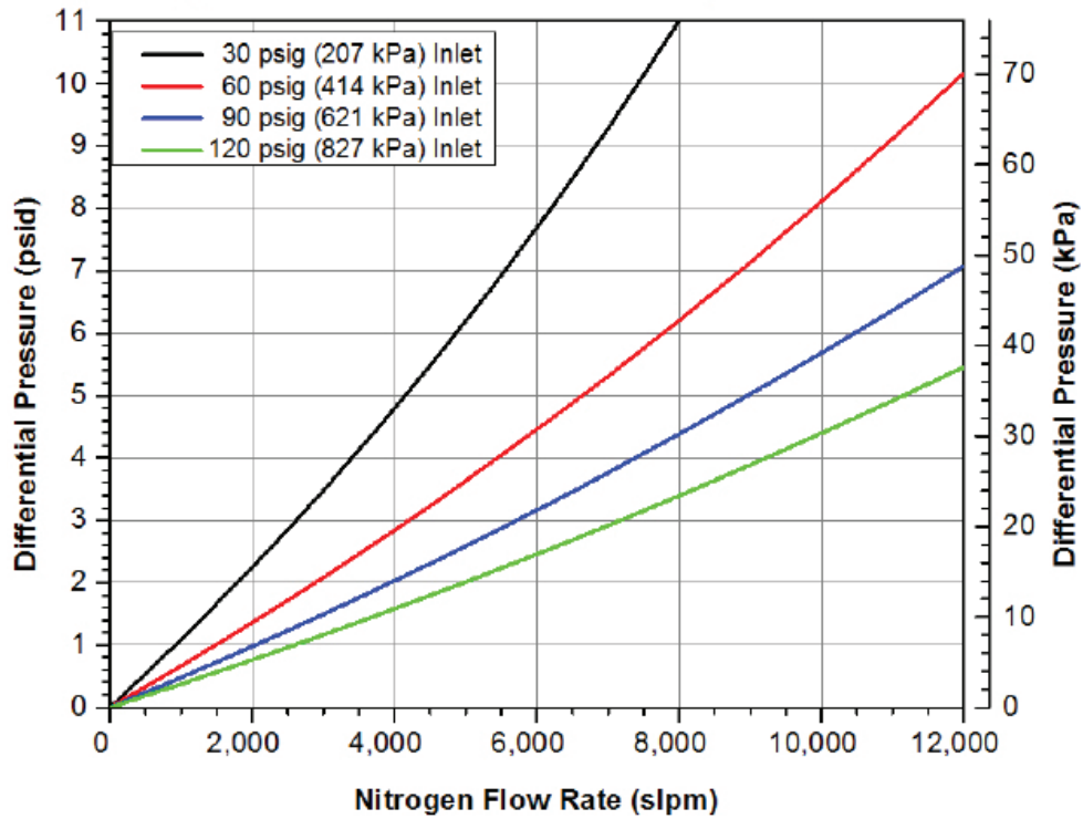
Mott BGF-315HF Flow Rate vs. Differential Pressure Typical Flow Curves as a Function of System Pressures
