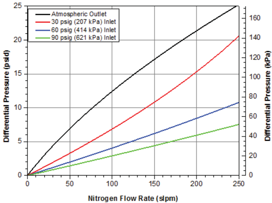
Mott POU-10-S Flow Rate vs. Differential Pressure Typical Flow Curves as a Function of System Pressures
