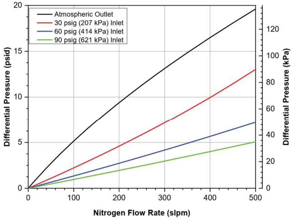
Mott GSP515H3F33 Flow Rate vs. Differential Pressure Typical Flow Curves as a Function of System Pressures
