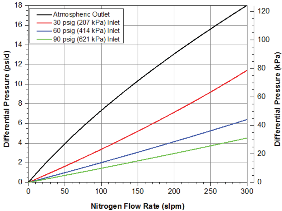
Mott GSP515H1 Flow Rate vs. Differential Pressure Typical Flow Curves as a Function of System Pressures
