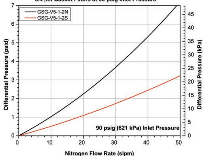
Mott GSG-V5-1-2N and GSG-V5-1-2S Flow Rate vs. Differential Pressure 0.4 \mu m Gasket Filters at 90 psig Inlet Pressure
