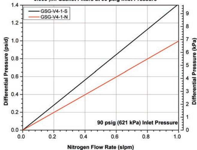
Mott GSG-V4-1-N and GSG-V4-1-S Flow Rate vs. Differential Pressure 0.003 \mu m Gasket Filters at 90 psig Inlet Pressure
