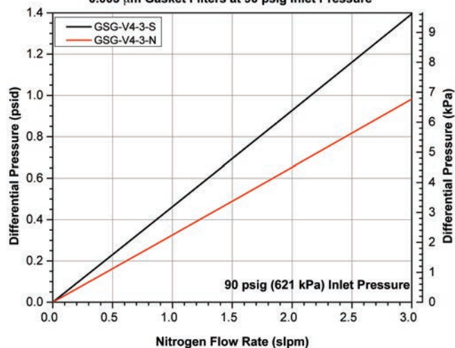
Mott GSG-V4-3-N and GSG-V4-3-S Flow Rate vs. Differential Pressure 0.003 \mu m Gasket Filters at 90 psig Inlet Pressure
