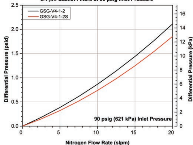
Mott GSG-V4-1-2 and GSG-V4-1-2S Flow Rate vs. Differential Pressure 0.4 \mu m Gasket Filters at 90 psig Inlet Pressure
