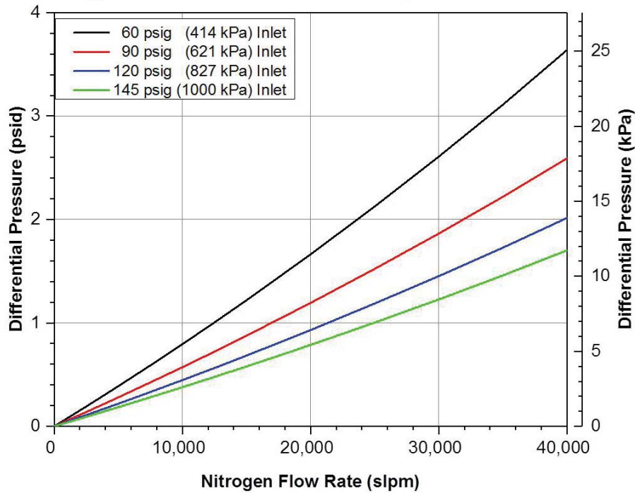
Mott BGF-615H Flow Rate vs. Differential Pressure Typical Flow Curves as a Function of System Pressures
