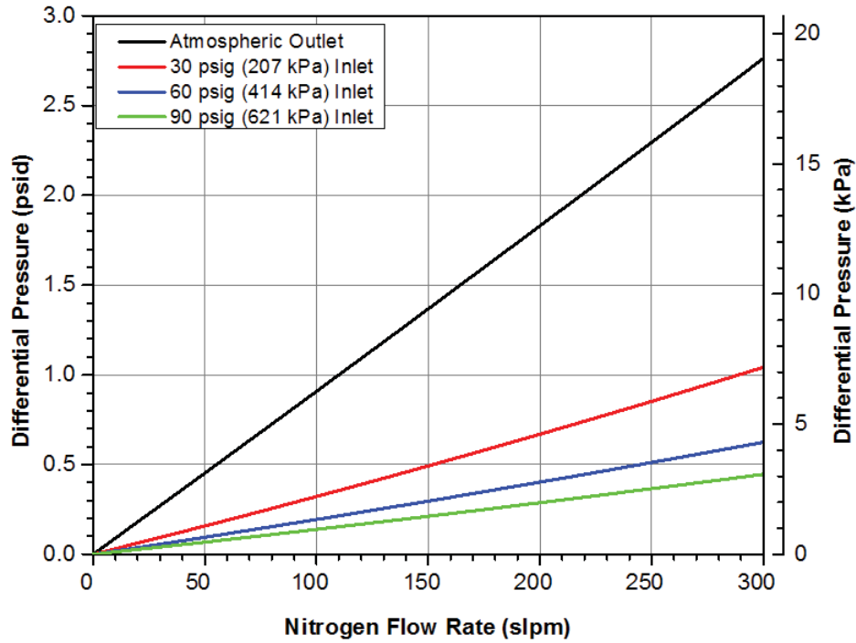
Mott FLT515 Flow Rate vs. Differential Pressure Typical Flow Curves as a Function of System Pressures
