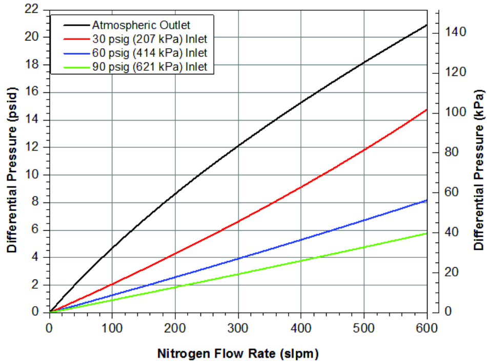
Mott POU-30-S Flow Rate vs. Differential Pressure Typical Flow Curves as a Function of System Pressures
