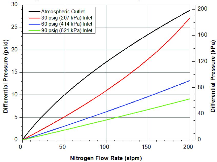
Mott POU-10-H Flow Rate vs. Differential Pressure Typical Flow Curves as a Function of System Pressures
